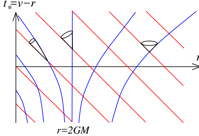
Figure 32. The Finkelstein diagram in ingoing coordinates. Ingoing null geodesics are shown in red, outgoing in blue. Inside the horizon at r = 2GM , outgoing geodesics do not go out.
