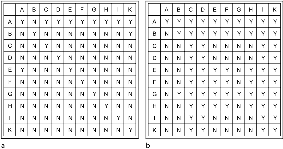
Fig. 2.7. Comparability of equilibrium states. Results of two fictitious series of experiments in which the adiabatic accessibility of states has been investigated. Which of the two tables violates the comparison principle and cannot therefore be described by an entropy function?
