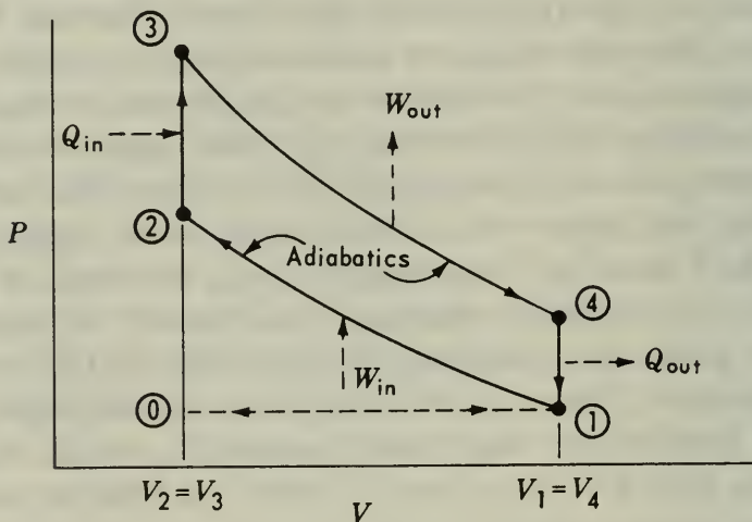
Figure 3-1 Otto engine cycle.
