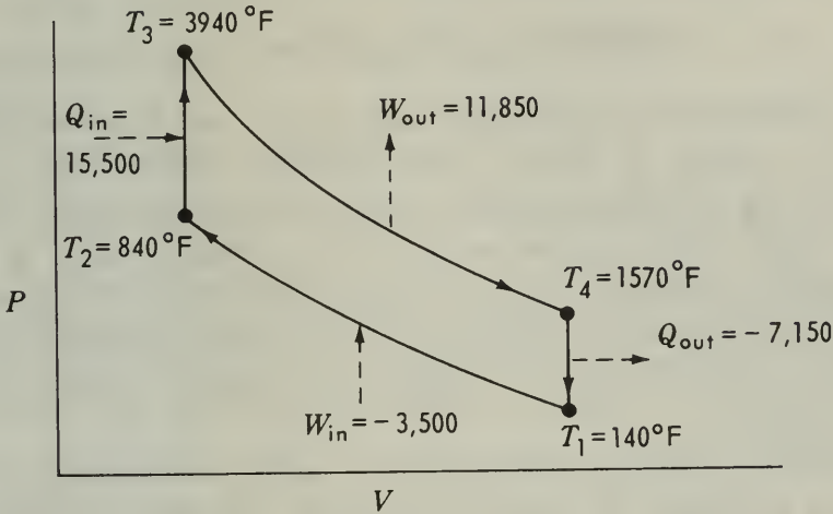
Figure 3-2 Results for idealized Otto cycle.
