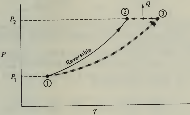
Figure 5-8 Adiabatic compression.
