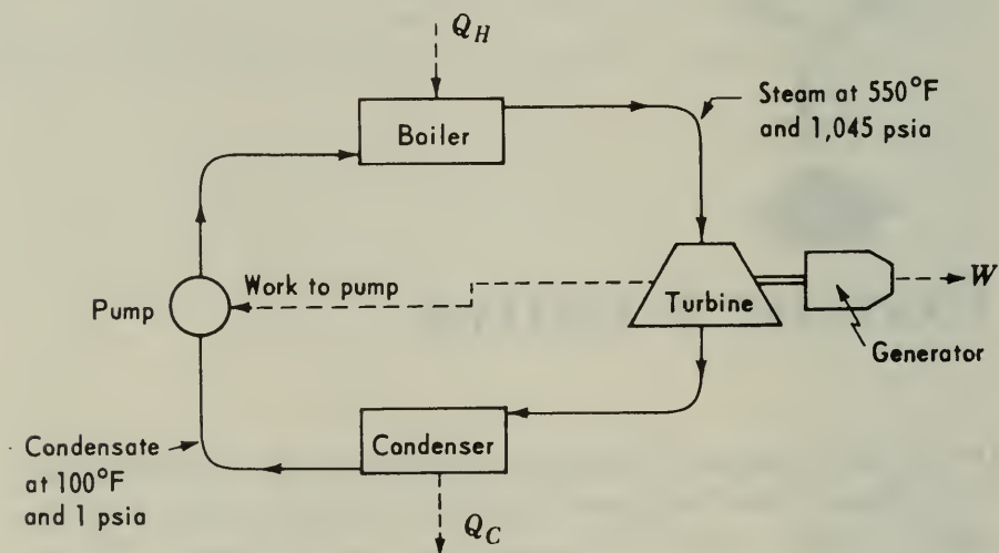
Figure 4-1 Steam cycle for stationary power plant.
