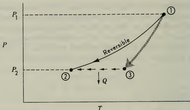
Figure 5-7 Adiabatic expansion.
