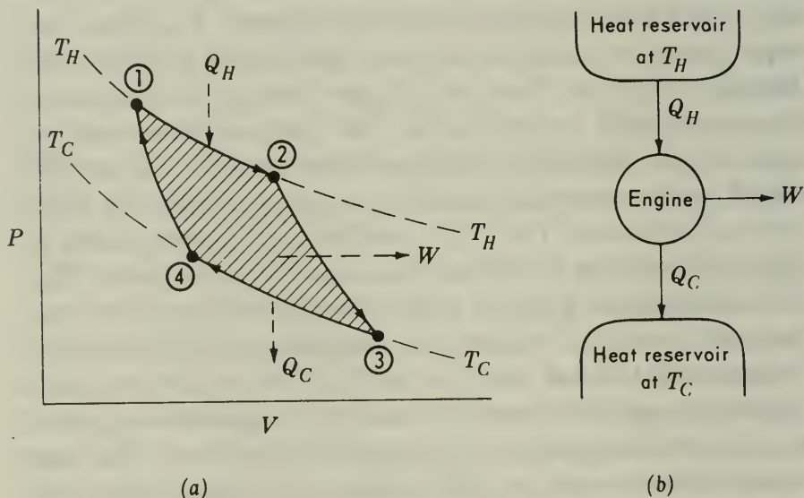
Figure 3-3 The Carnot engine cycle.
