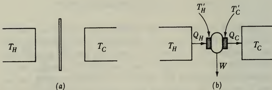
Figure 5-2 Thermal process.
