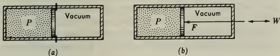
Figure 5-1 Adiabatic mechanical process.
