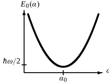
Figure 9.4 Shape of E_0(\alpha) = \hbar^2\alpha/(2m) + m\omega^2/(8\alpha) .
