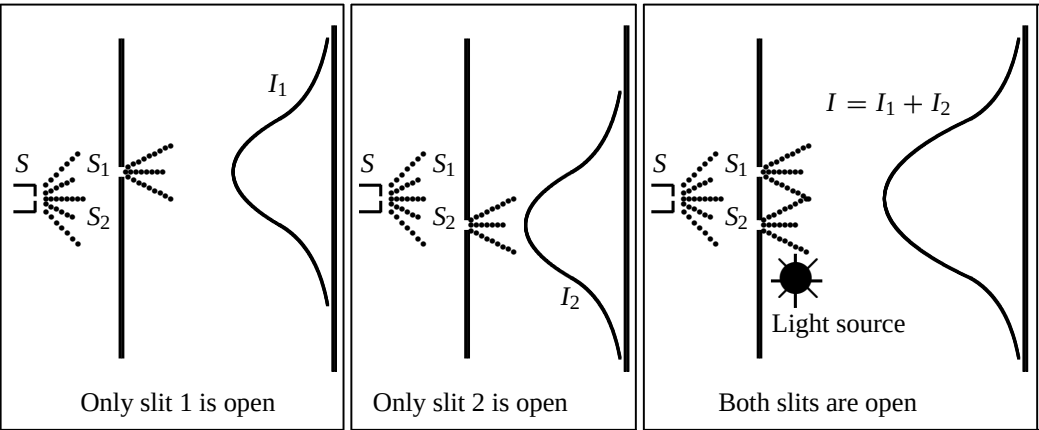
Figure 1.11 The double-slit experiment: S is a source of electrons. A light source is placed behind the wall containing S_1 and S_2 . When both slits are open, the interference pattern is destroyed and the total intensity is I = I_1 + I_2 .
