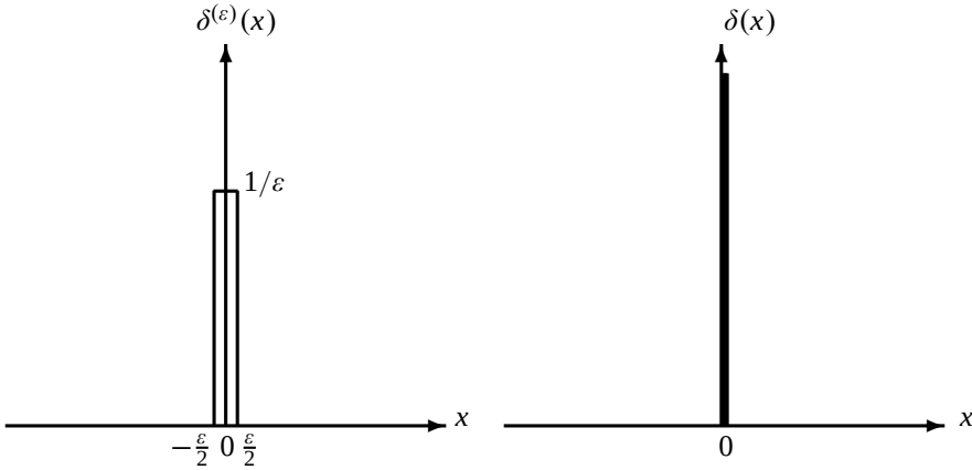
Figure A.1 The delta function \delta(x) as defined by \delta(x) = \lim_{\varepsilon \rightarrow 0} \delta^{(\varepsilon)}(x) .
