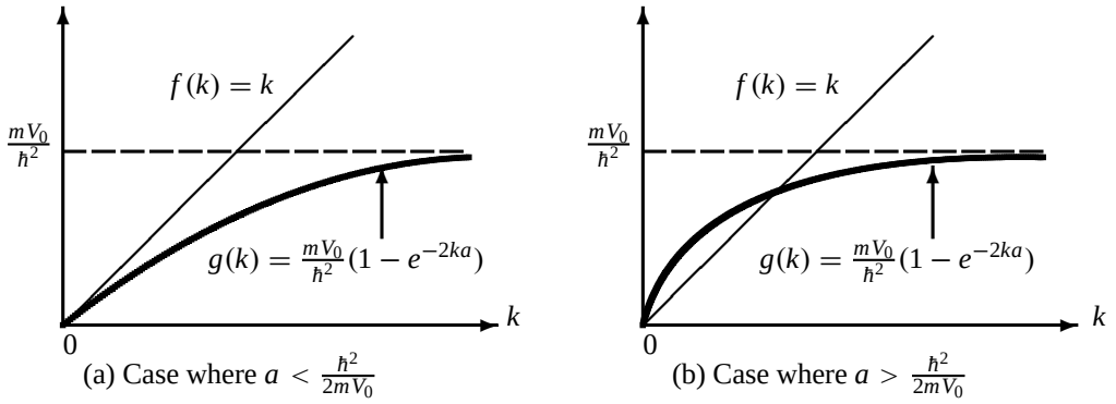
Figure 4.14 Graphical solutions of f(k) = g(k) or k = (mV_0/h^2)(1 - e^{-2ka}) . If the slope of g(k) is smaller than 1, i.e., a < h^2/(2mV_0) , no bound state will exist, but if the slope of g(k) is greater than 1, i.e., a > h^2/(2mV_0) , there will be only one bound state.
