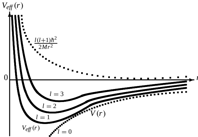
Figure 6.1 The effective potential V_{\text{eff}}(r) = V(r) + \frac{\hbar^2 l(l+1)}{2Mr^2} corresponding to several values of l : l = 0, 1, 2, 3 ; V(r) is an attractive central potential, while \frac{\hbar^2 l(l+1)}{2Mr^2} is a repulsive (centrifugal) potential.
