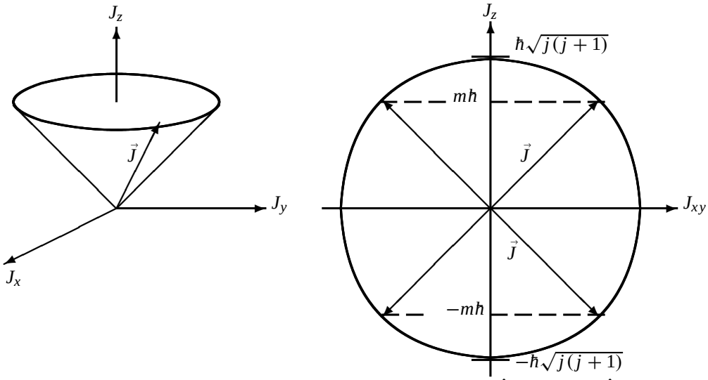
Figure 5.1 Geometrical representation of the angular momentum \hat{J} : the vector \hat{J} rotates along the surface of a cone about its axis; the cone's height is equal to mh , the projection of \hat{J} on the cone's axis. The tip of \hat{J} lies, within the J_z J_{xy} plane, on a circle of radius h\sqrt{j(j+1)} .
