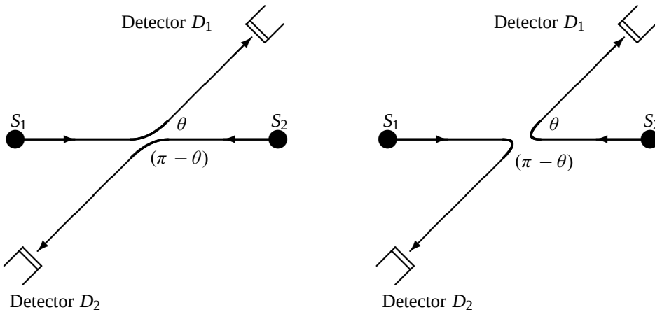
Figure 8.1 When scattering two identical particles in the center of mass frame, it is impossible to forecast with certainty whether the particles scatter according to the first process or to the second. For instance, we cannot tell whether the particle fired from source S_1 will make it to detector D_1 or to D_2 .
